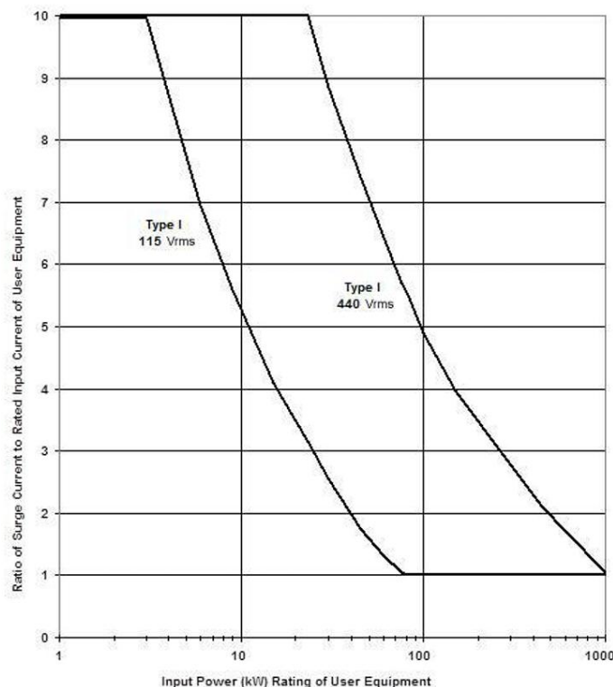
Figure 6: Ratio of Inrush current (surge current) to rated current for low voltage loads (MIL-STD-1399-300-1)
